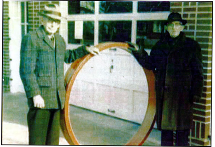
A photo of the Cape May Court House Fire Company Chief John Ross and Chief Burton Carson standing next to their steel locomotive rim that was used to alert firefighters.
