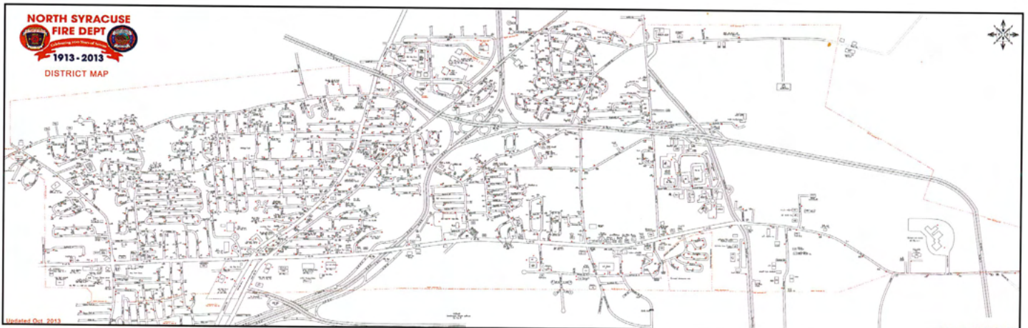
The North Syracuse Fire Department district map from 2013.
